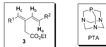
Figure 1. Structures of 3 and PTA.
