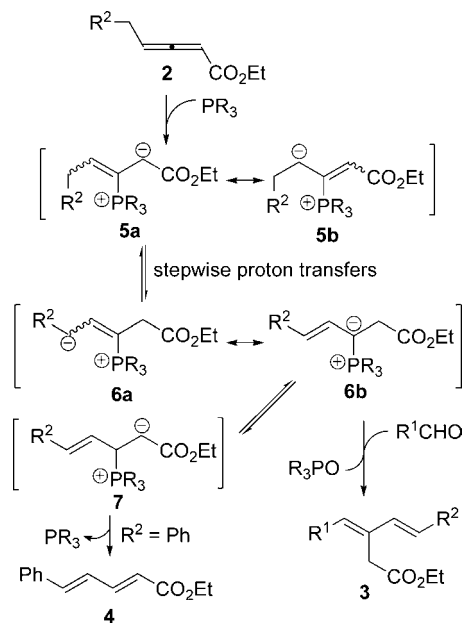
Scheme 1. Proposed Mechanism of Formation of 3 and 4
